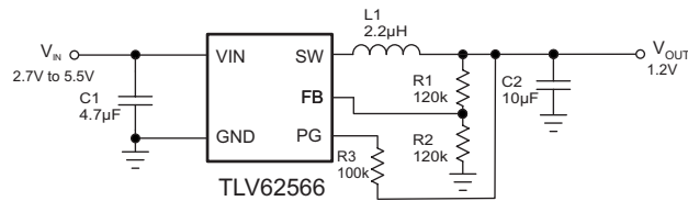
Figure 28. TLV62566 1.2-V Output Application
