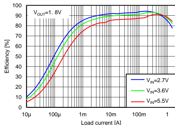
Figure 2. TLV62565 Efficiency, 1.8 V OUT
