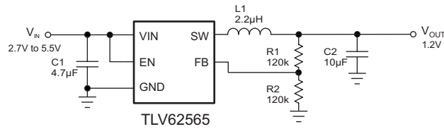
Figure 25. TLV62565 1.2-V Output Application
