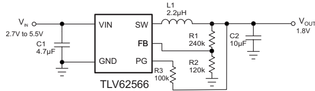
Figure 29. TLV62566 1.8-V Output Application
