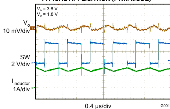
TYPICAL APPLICATION (PWM MODE)
