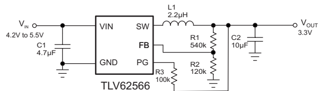
Figure 30. TLV62566 3.3-V Output Application
