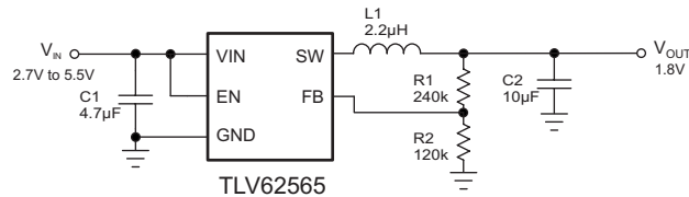
Figure 26. TLV62565 1.8-V Output Application
