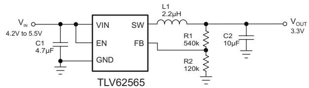
Figure 27. TLV62565 3.3-V Output Application
